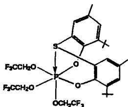
C 7 ( ^{31}\text{P} = -82.3 ppm)
