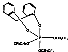
F 3 ( ^{31}\text{P} = -78.3 ppm)
