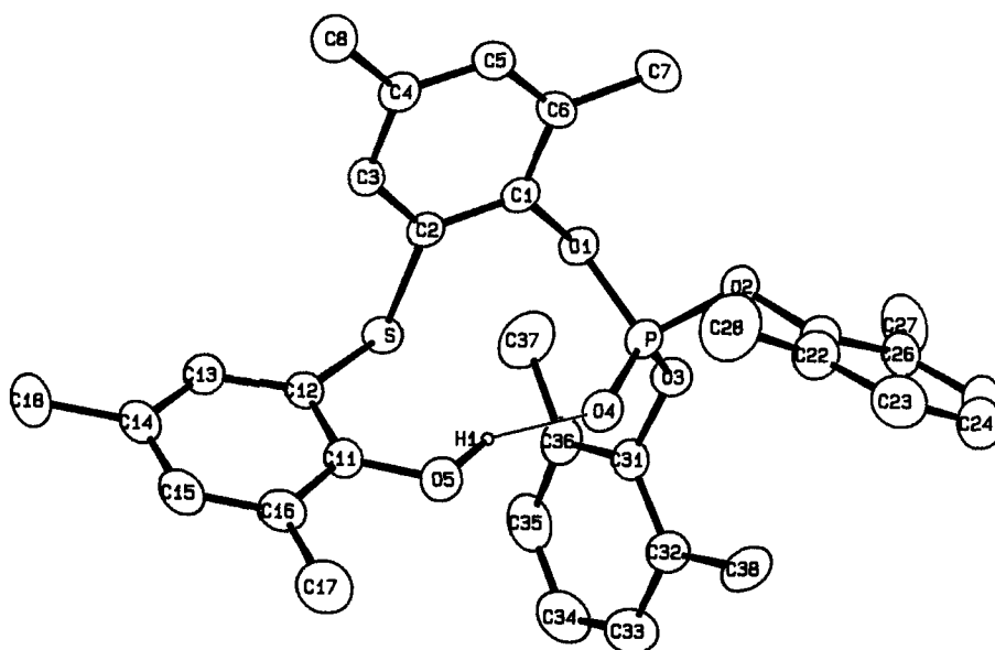
FIGURE 3 ORTEP plot of S(\text{Me}_2\text{C}_6\text{H}_2)_2(\text{OH})\text{OP}(\text{O})(\text{OXyl})_2 , 4 , with thermal ellipsoids at the 30% probability level. Hydrogen atoms, except for H1 which is shown as a sphere of arbitrary radius, are omitted for clarity. The hydrogen-bonding interaction is shown as a narrow line.
