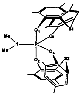
1 ( ^{31}\text{P} = -76.5 ppm)
