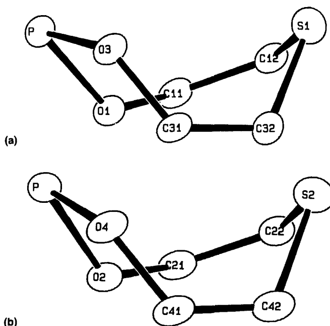
FIGURE 2 ORTEP plots showing the conformations of the eight-membered rings in 1: (a, top) Ring containing S1; (b, bottom) ring containing S2.
