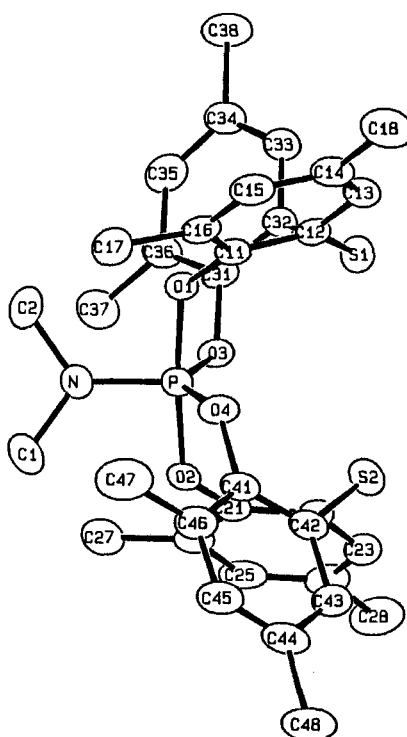
FIGURE 1 ORTEP plot of [\text{S}(\text{Me}_2\text{C}_6\text{H}_2\text{O})_2]_2\text{PNMe}_2 , 1 , with thermal ellipsoids at the 30% probability level. Hydrogen atoms are omitted for clarity.
